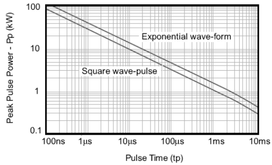
Figure 1. Non-repetitive peak pulse power rating curve
